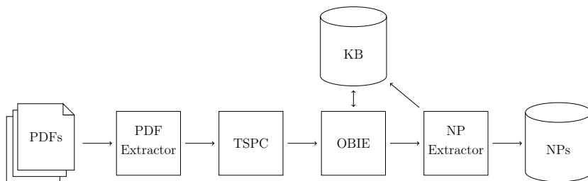
Fig. 3. Flow of the nanopublication extraction system
